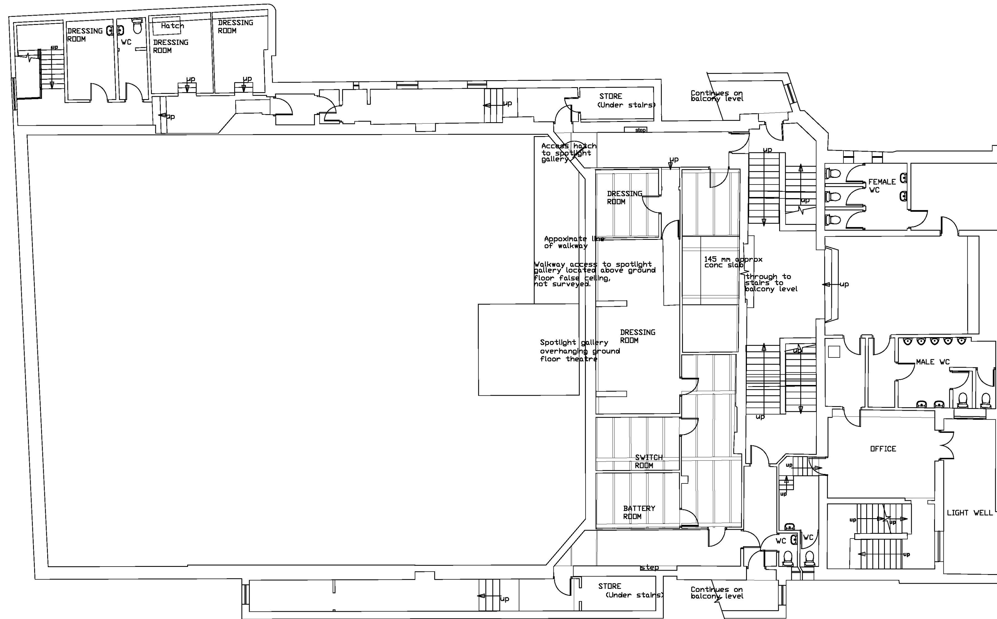
Existing Mezzanine Level Scale 1:100 @ A1
